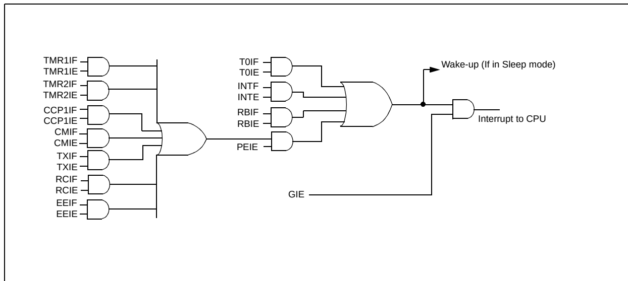
FIGURE 14-14: INTERRUPT LOGIC
