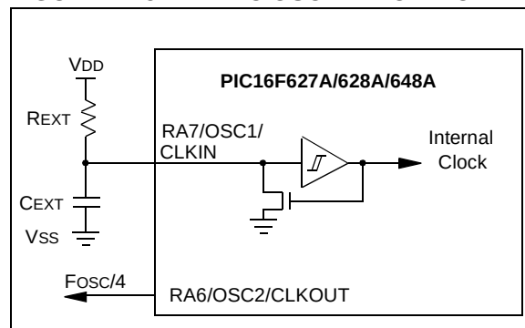
FIGURE 14-5: RC OSCILLATOR MODE
