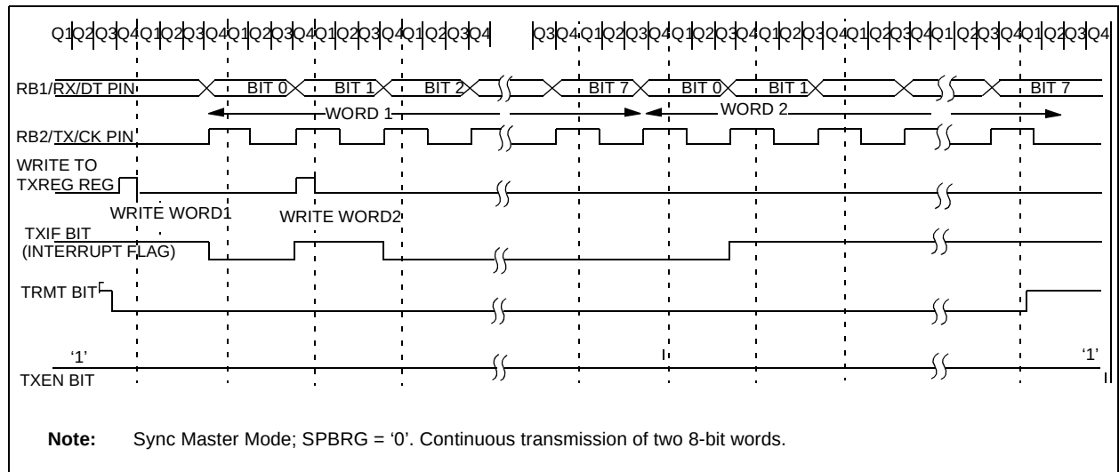
FIGURE 12-12: SYNCHRONOUS TRANSMISSION
